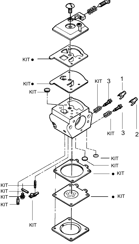
Carburetor Assembly – WT610 – #530071492
