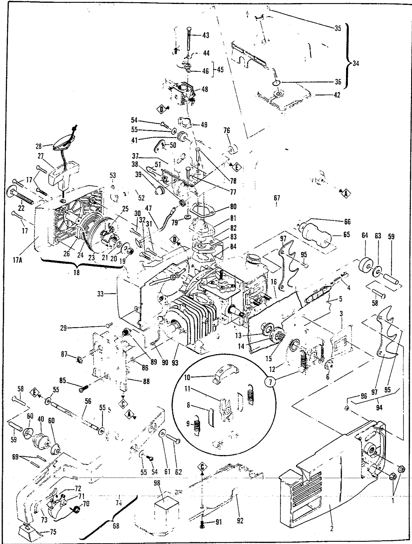
Figure 1 GENERAL ASSEMBLY
