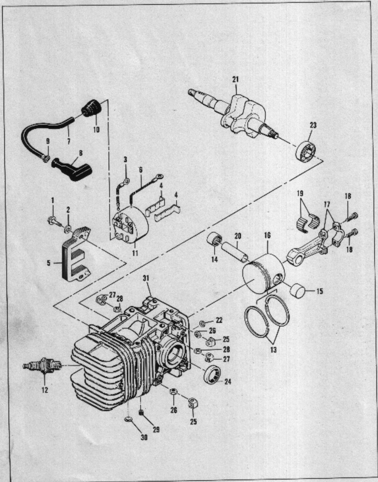
Figure 6. Powerhead Assembly
