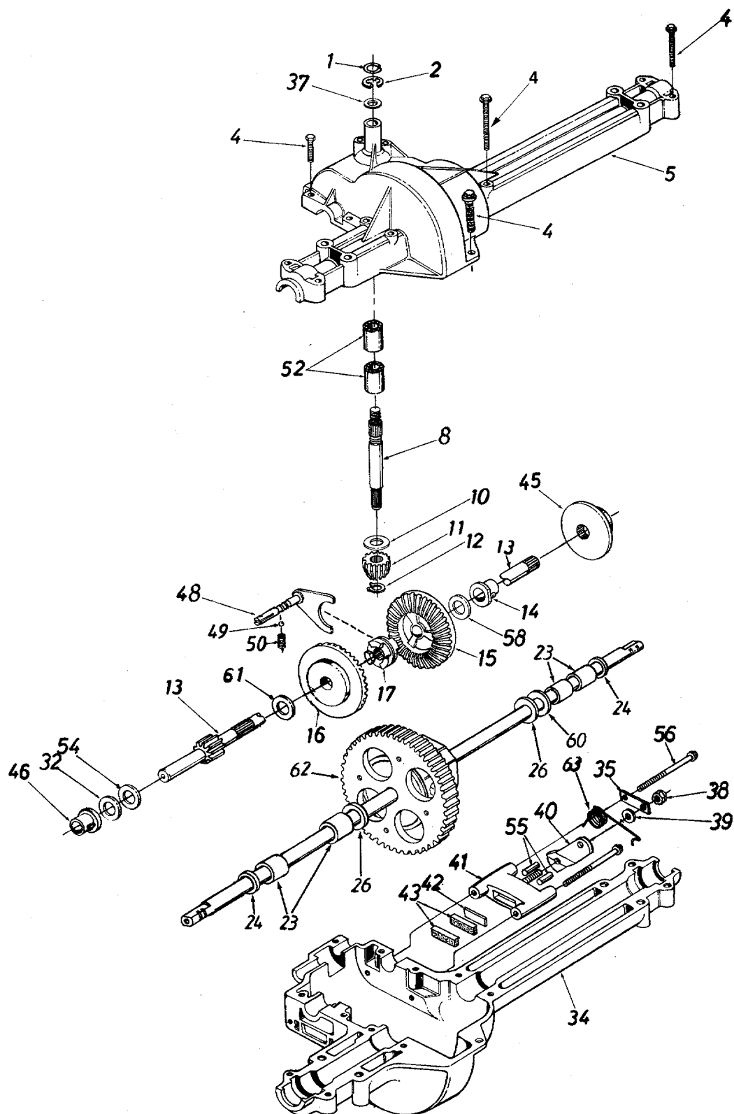
Single Speed Transaxle—R.H. Model 618-0163B
