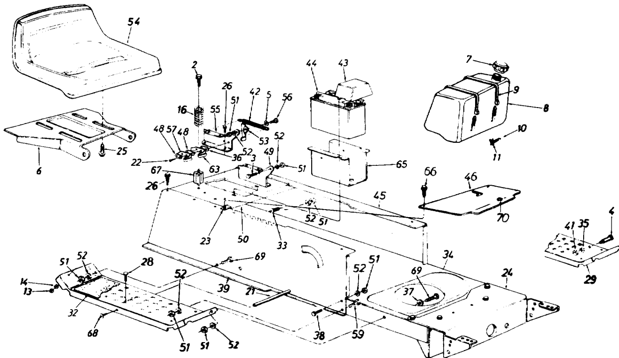
18 H.P. 42" AND 46" LAWN TRACTORS PARTS LIST FOR MODELS TMO-3400005 AND TMO-3500006
