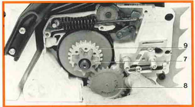
Top: Removing the drive worm Center: Circlip correctly fitted Bottom: Rim sprocket in position
