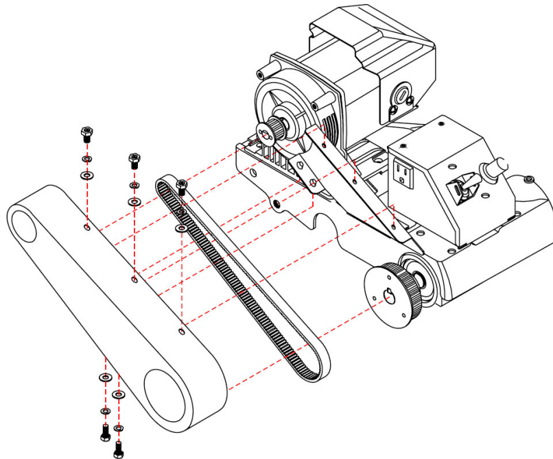
Belt Guard Removal
